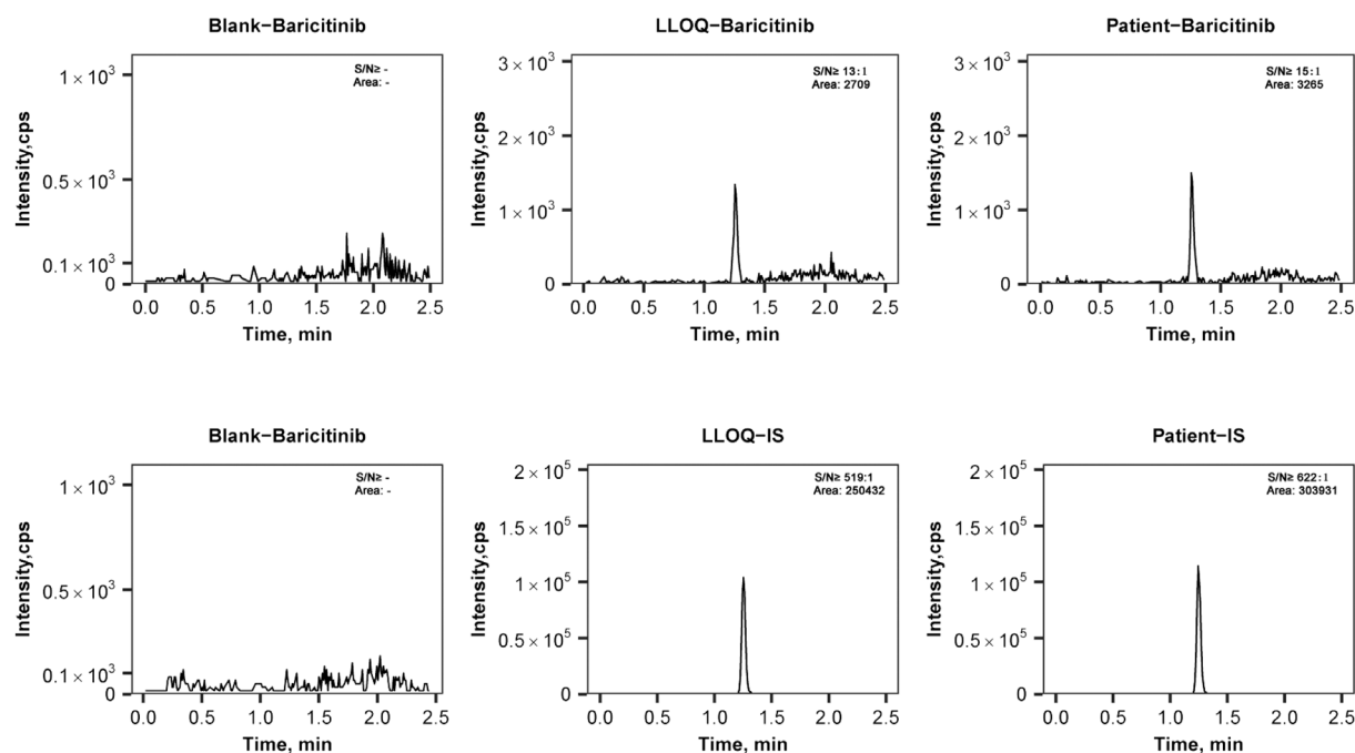
FIGURE 2. Typical MRM chromatograms of baricitinib and IS in double-blank plasma, LLOQ plasma sample, and plasma sample from patient (No. 4) collected immediately before (0 h) the second dosage administration.
