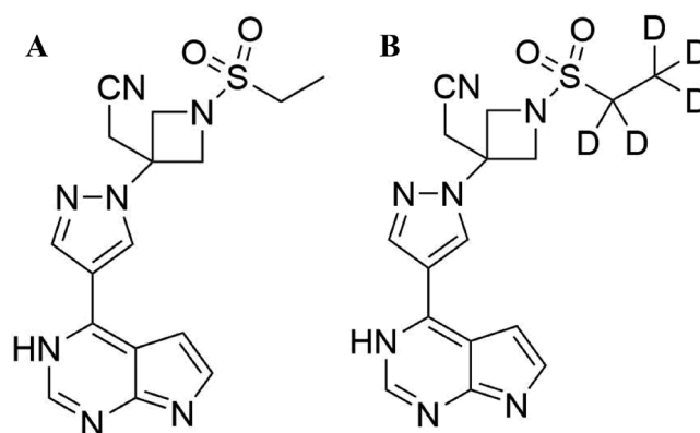
FIGURE 1. Chemical structure of baricitinib ( A ) and its isotopic IS ( B ).
